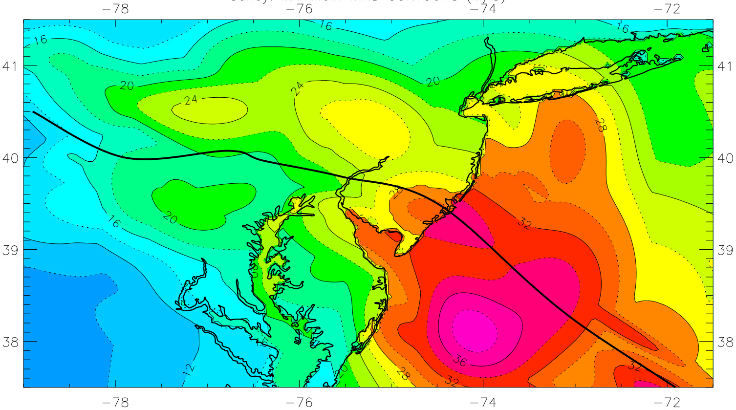
Sandy: MAXIMUM WIND CONTOURS (M/S)
